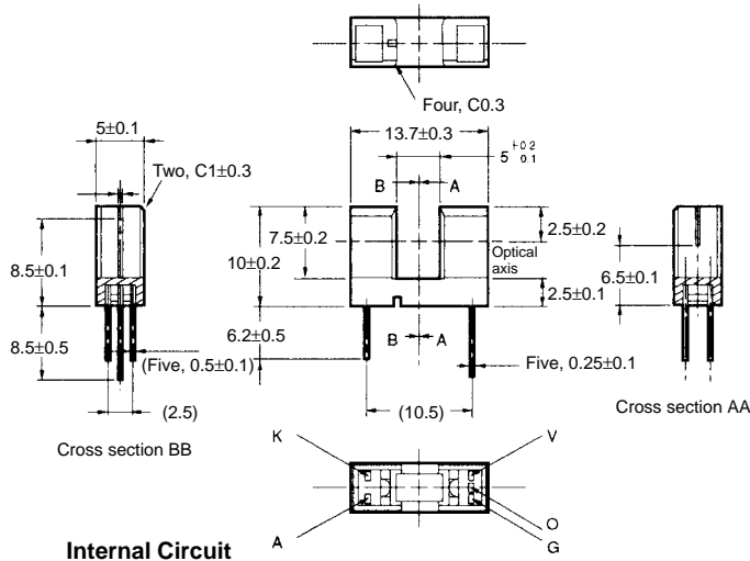
Internal Circuit
